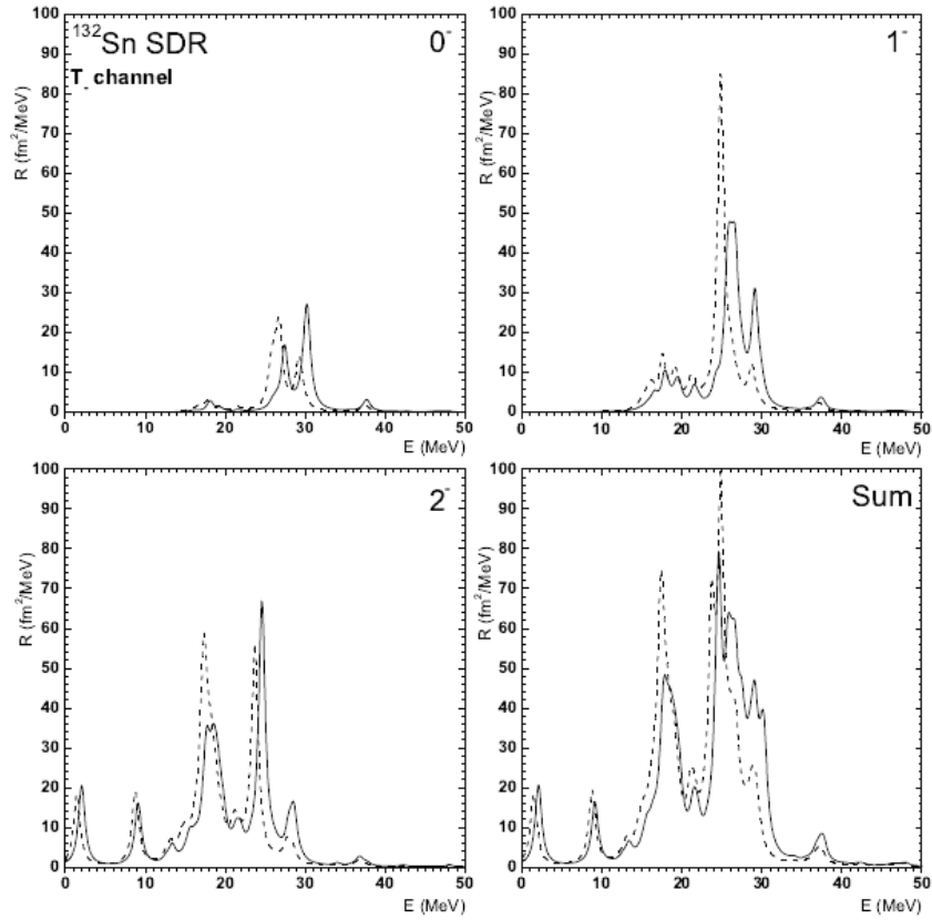
Fig. 1. Spin-dipole strength distributions in the T_ channel of the parent nucleus ^{132}\text{Sn} , calculated by using the force SGII [20]. The results with the FRSA for the p-h interaction (dashed lines), and with the full p-h interaction (solid lines) are shown.
